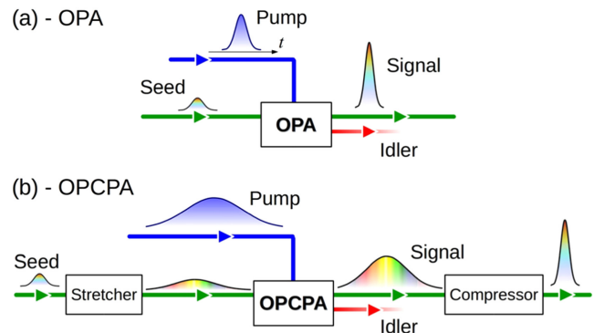
Figure 19. (a) Conceptual scheme of an ultrafast OPA; (b) conceptual scheme of an OPCPA.
